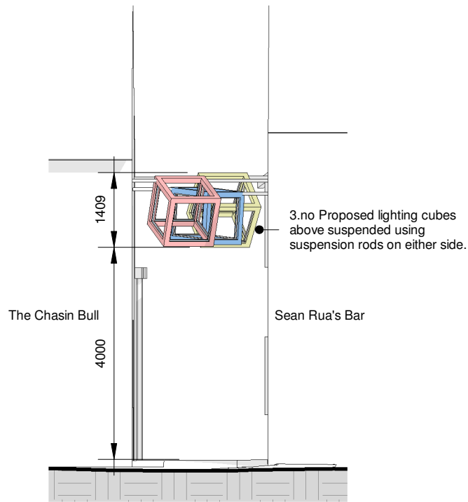
Main Street Elevation 1 : 100
