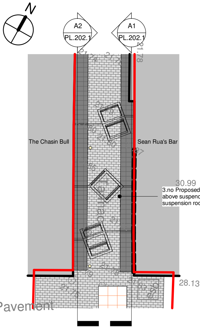
Lighting Cubes Site Plans 1 : 100
