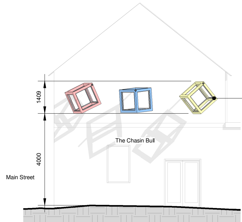
Lighting Cubes Elevation - A1 1 : 100
