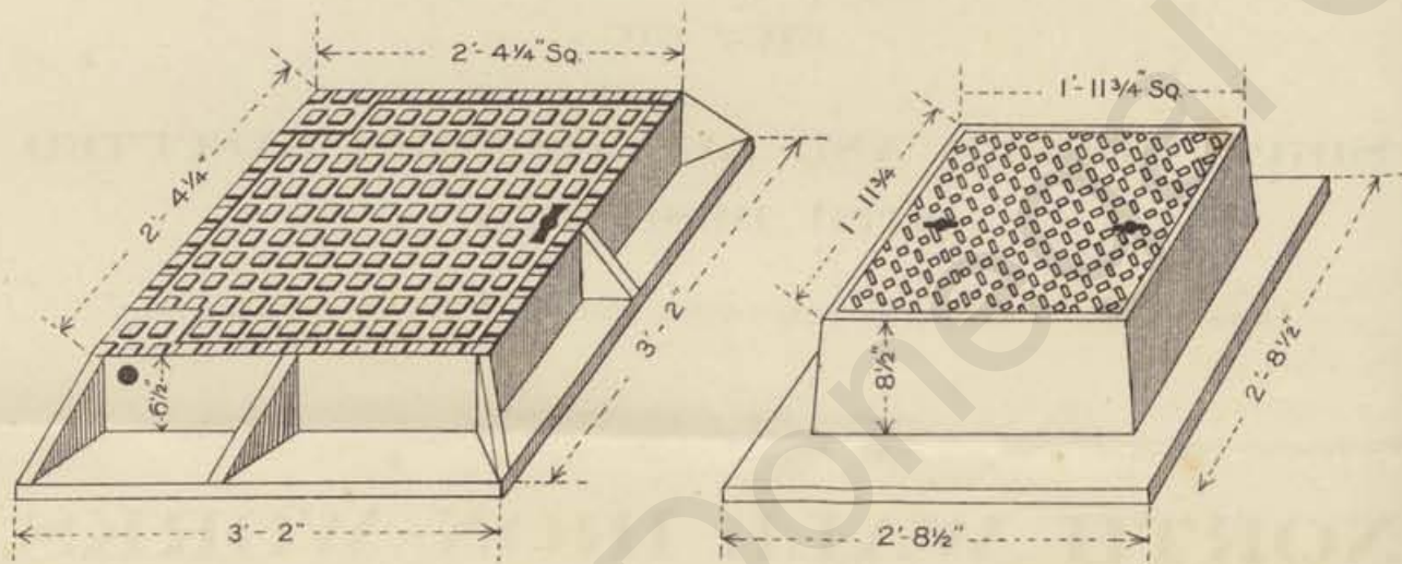
HINGED MANHOLE WITH LOCKING ARRANGEMENT.
