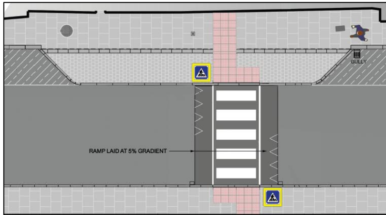
Typical Layout A. Proposed Pedestrian Crossing at Ped S1, Ped S2, Ped B1 & Ped B2.
