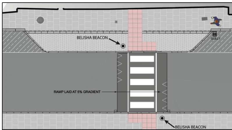
Typical Layout B. Proposed Pedestrian Crossing at Ped B4.
