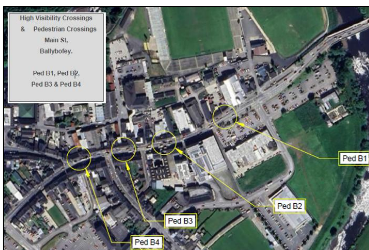
N15 Main St, Ballybofey - Scheme Location Showing Proposed Works.
